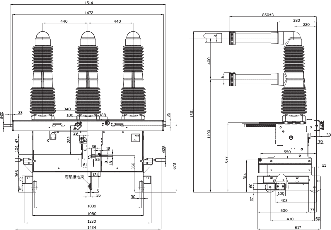
手车式40.5 kV 1600~2500A...31.5 kA P440
